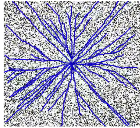
Figure 13: Complex 512 × 512 with 200 agents. Goal is in center of map, and computed paths are shown in blue. Every black area is an obstacle.
